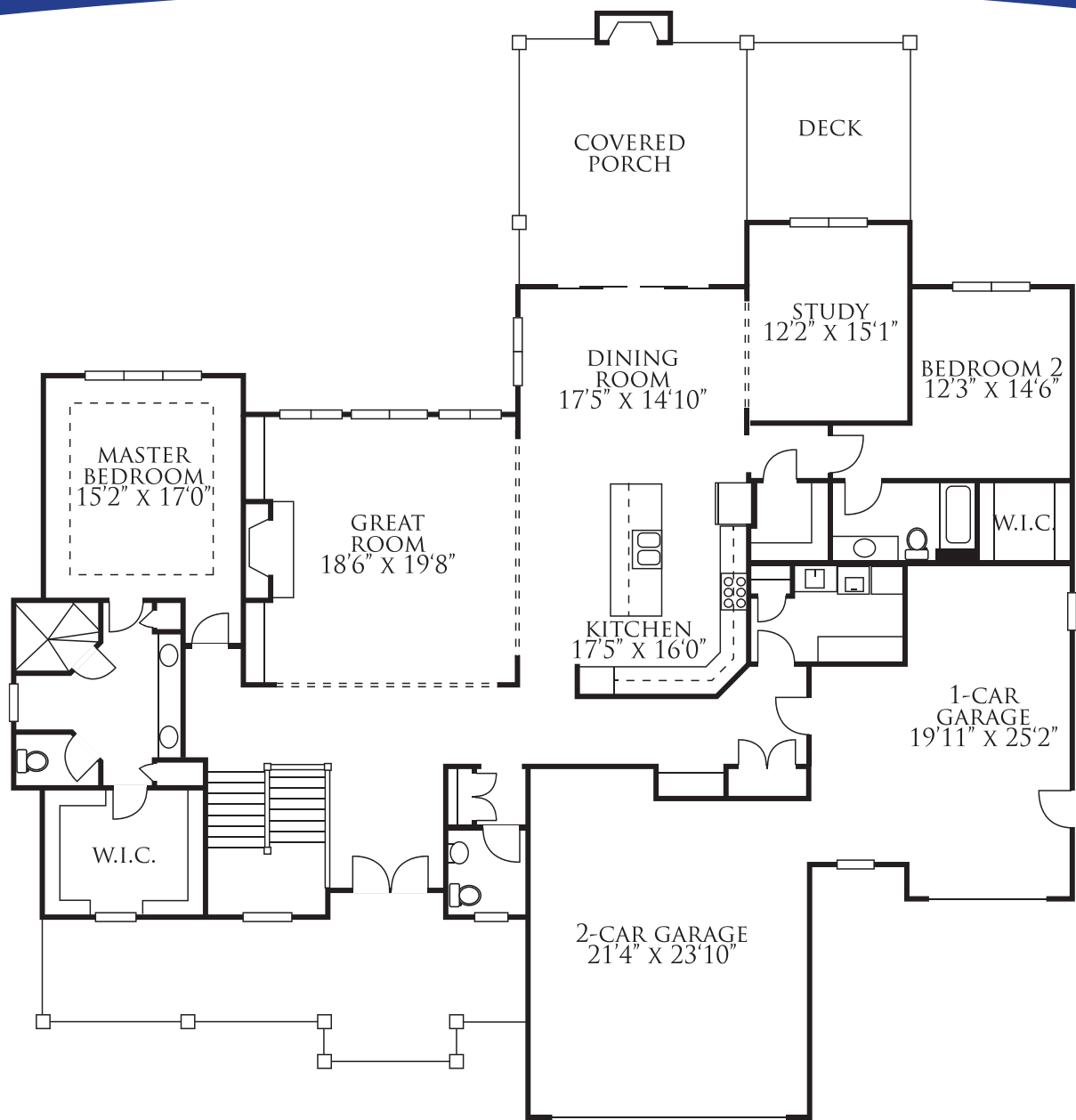
FIRST FLOOR
