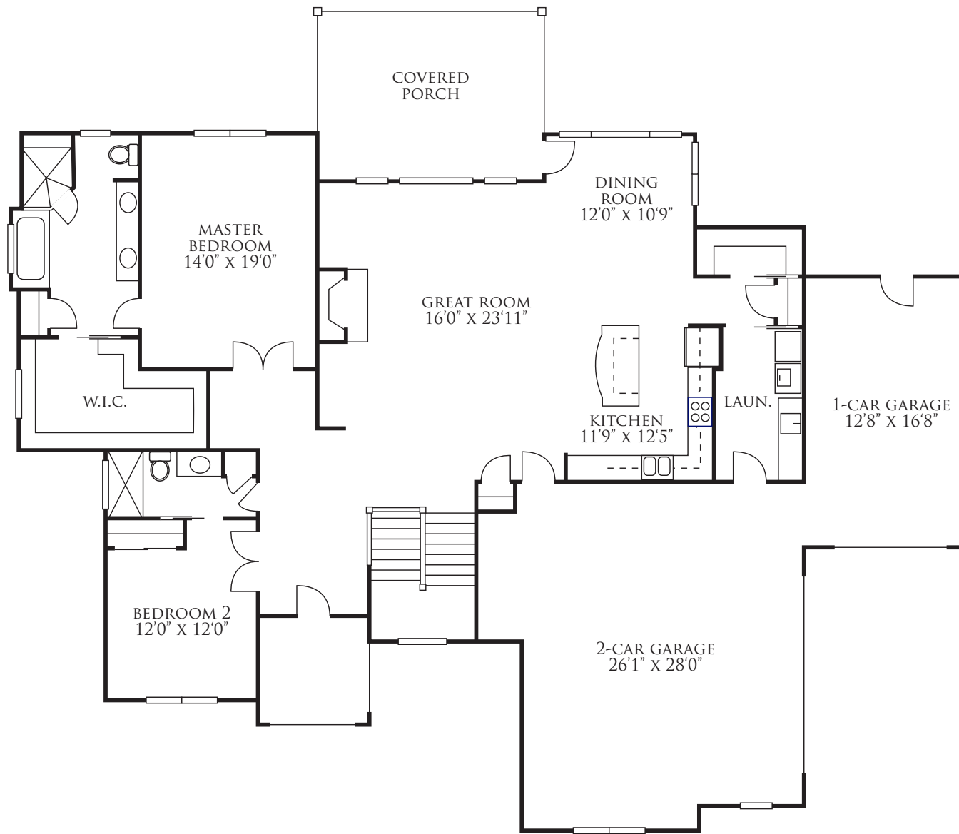
FIRST FLOOR
